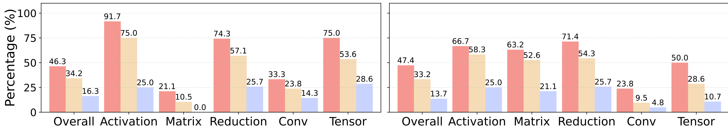
(a) MNN
